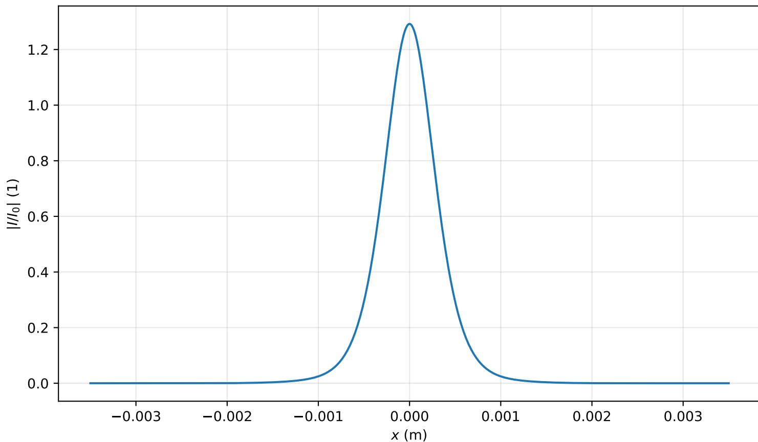
Intensity profile I(x, y = 0, z = 2.149m)/I_0 , P_{in}=0.8P_{cr} , artificial time
